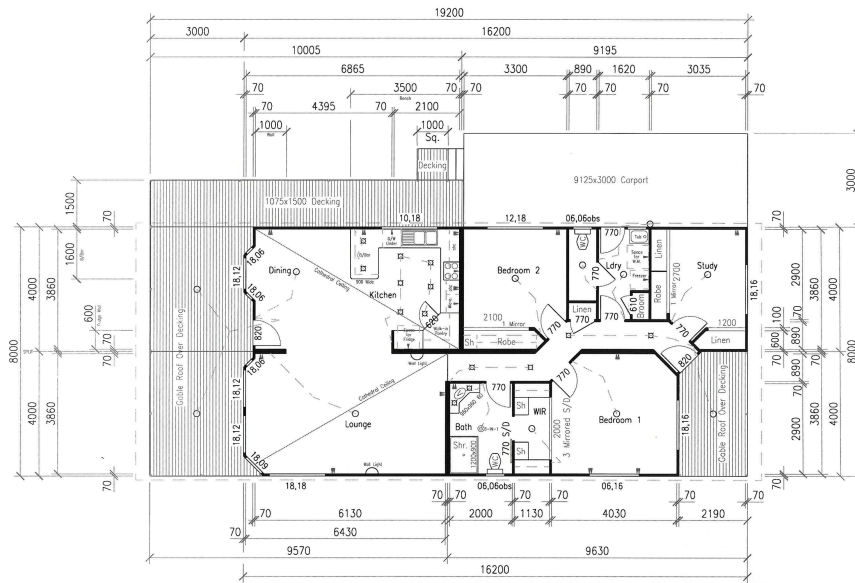
FLOOR PLAN PROPOSED TWO BEDROOM + STUDY DWELLING
